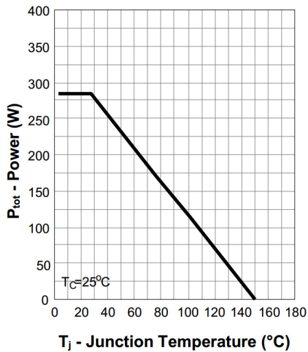
1. Power Capability
