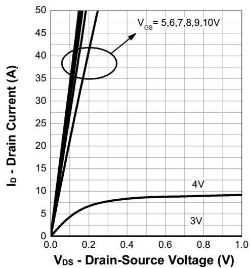
5. Output Characteristics
