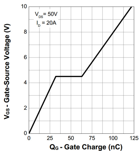
12. Gate Charge
