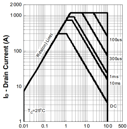
3. Safe Operating Area
