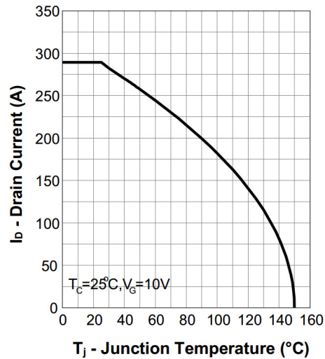
2. Current Capability
